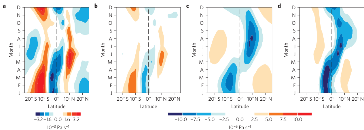
Figure 3 | Circulation change and decomposition of precipitation change. a-d, \Delta\omega at 500 hPa (a); dynamic ( \Delta\omega \cdot \bar{q} ) (b) and thermodynamic ( \bar{\omega} \cdot \Delta q ) (c) components of rainfall change and their sum (d).
