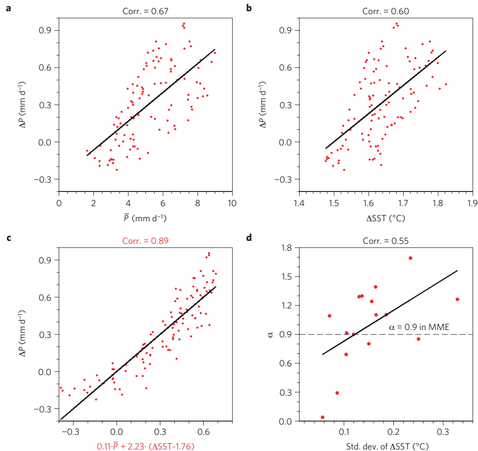
Figure 4 | Relationship of precipitation change to mean precipitation, SST change pattern and their linear combination. a–c , Scatter plots of MME precipitation change with mean precipitation ( a ), SST change ( b ) and their linear combination (equation (2)); c ) in 10^{\circ}\text{S} – 10^{\circ}\text{N} through the seasonal cycle. The solid line indicates the linear fit, with the correlation coefficient shown at the top. d , The multi-variant regression analysis is also performed for each model, and the ratio \alpha is shown in relation to the spatial standard deviation of \Delta\text{SST} .
