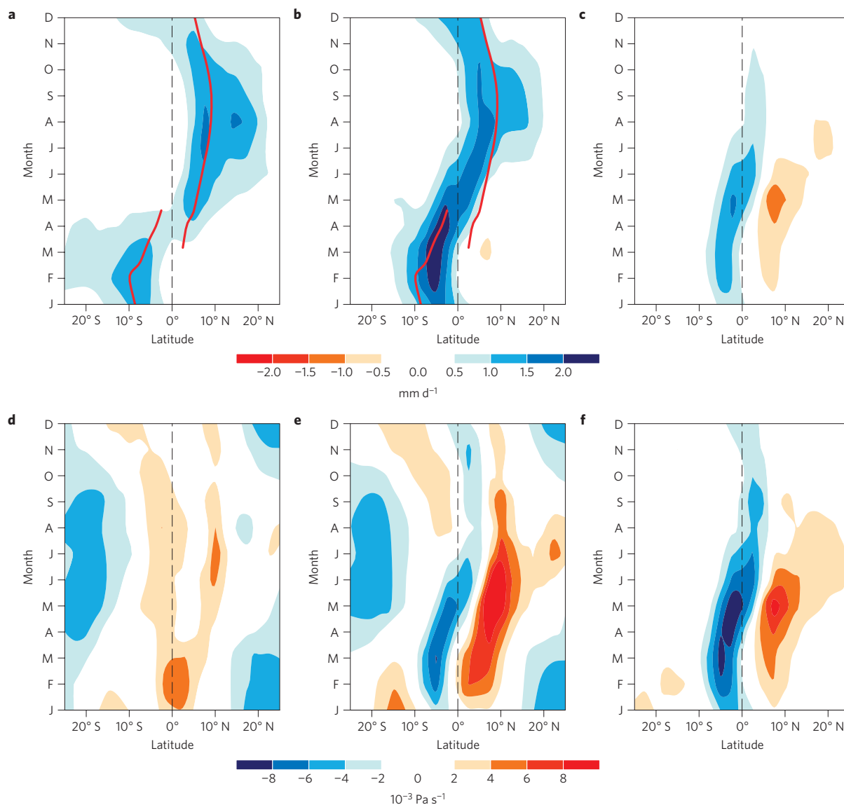
Figure 2 | Seasonal cycle of precipitation and circulation changes in SUSI and SPSI runs. a-c, \Delta P in SUSI (a) and SPSI (b) runs, and their difference (c). d-f, The same as in a-c but for pressure velocity \Delta\omega at 500 hPa. The solid red lines in a,b mark the latitude of the climatological precipitation maximum in the control. The SPSI results are scaled by the 20^\circ \text{S} - 20^\circ \text{N} mean \Delta \text{SST} to match SUSI.
