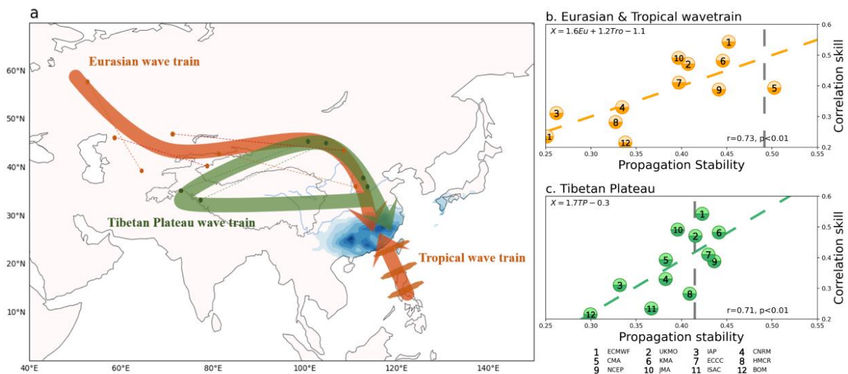
Fig. 6. Propagation stability of EASM ISV origins. a Schematic diagram of EASM ISV origins (arrows) from Eurasian and tropical wave trains for well-predicted (orange) ISV events, and from a western Tibetan Plateau wave train for poorly-predicted (green) events. The preceding upper-tropospheric cyclonic–anticyclonic centers (connected by dashed lines) and convection centers from Day -12 to Day 0 on Fig. 5 are indicated by dots and clouds, respectively. b Relationship between the seven-day leading prediction skill of weekly EASM precipitation index and propagation stability of the combination (through a multiple linear regression) of Eurasian and tropical wave trains in all 12 S2S models. Orange dashed line shows the linear regression with a significant correlation coefficient ( r ) and p -value. Observed propagation stability from 1979 to 2021 is also marked by a gray dashed line for reference. c Same as b , but for the western Tibetan Plateau wave train.
