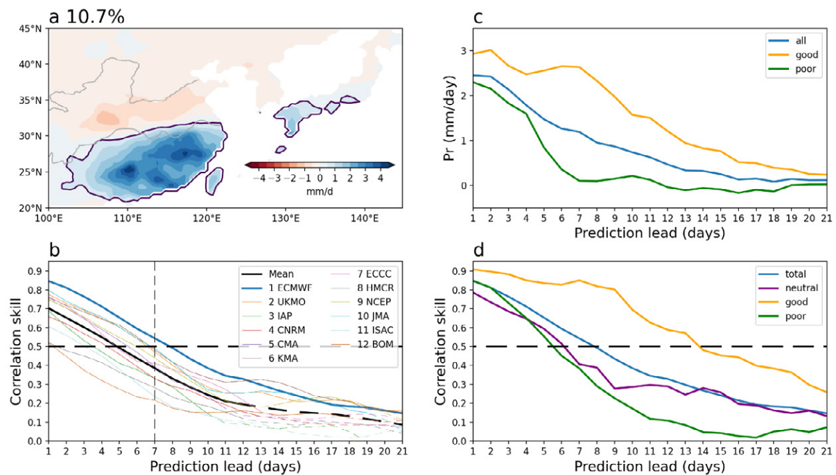
Fig. 1. EASM ISV and its prediction skill. a Leading mode of EASM ISV represented by the first EOF pattern of 12–40-day bandpass filtered EASM ( 20^{\circ} – 45^{\circ} N, 100^{\circ} – 145^{\circ} E) land precipitation anomalies in CPC observation from 1979 to 2021. The upper and lower gray lines denote the Yellow and Yangtze rivers, respectively. The purple contour delineates the wet EASM regions with precipitation anomalies > 0.5 \text{ mm day}^{-1} . The percentage variance explained by this leading mode is marked on the panel. b Prediction skill of weekly EASM precipitation index for 12 S2S models (colored lines) as a function of prediction lead days for their respective validation periods (Table 1). Black line denotes the multi-model mean. Solid lines denote significant ( p < 0.01 ) skills. c ECMWF predicted event amplitude ( \text{mm day}^{-1} ) of EASM ISV averaged for all ISV events (blue line), well-predicted events (orange line), and poorly-predicted events (green line). d ECMWF prediction skill of weekly EASM precipitation index for all weeks (blue line, same as in b ), weeks controlled by well-predicted (orange line) or poorly-predicted (green line) ISV events, and weeks without any effect from ISV events (purple line).
