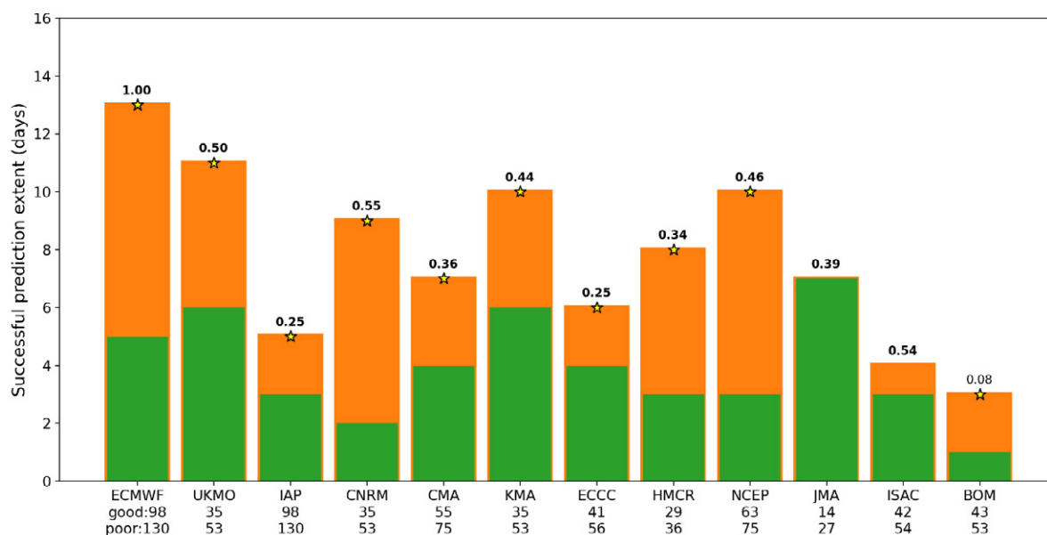
Fig. 4. ISV event-dependent sub-seasonal prediction skill. Longer prediction extent for skillful prediction of weekly EASM precipitation index from control by well-predicted (orange bars) than by poorly-predicted (green bars) events in all 12 S2S models. These well- and poorly-predicted ISV events are defined based on ECMWF prediction, and only the periods that overlap with ECMWF prediction are analyzed in the other models. Stars indicate significant improvement ( p < 0.05 ) based on the Monte Carlo method with 10,000 iterations. The prediction extent is defined by the last day on which the correlation coefficient is > 0.5 . Correlation (number over the bar) of seven-day leading prediction scores for all overlapped ISV events between ECMWF and each of the other models is also listed, with significant ( p < 0.05 ) correlations highlighted in bold type. The numbers of overlapped well- and poorly-predicted ISV events are listed below the name of each model.
