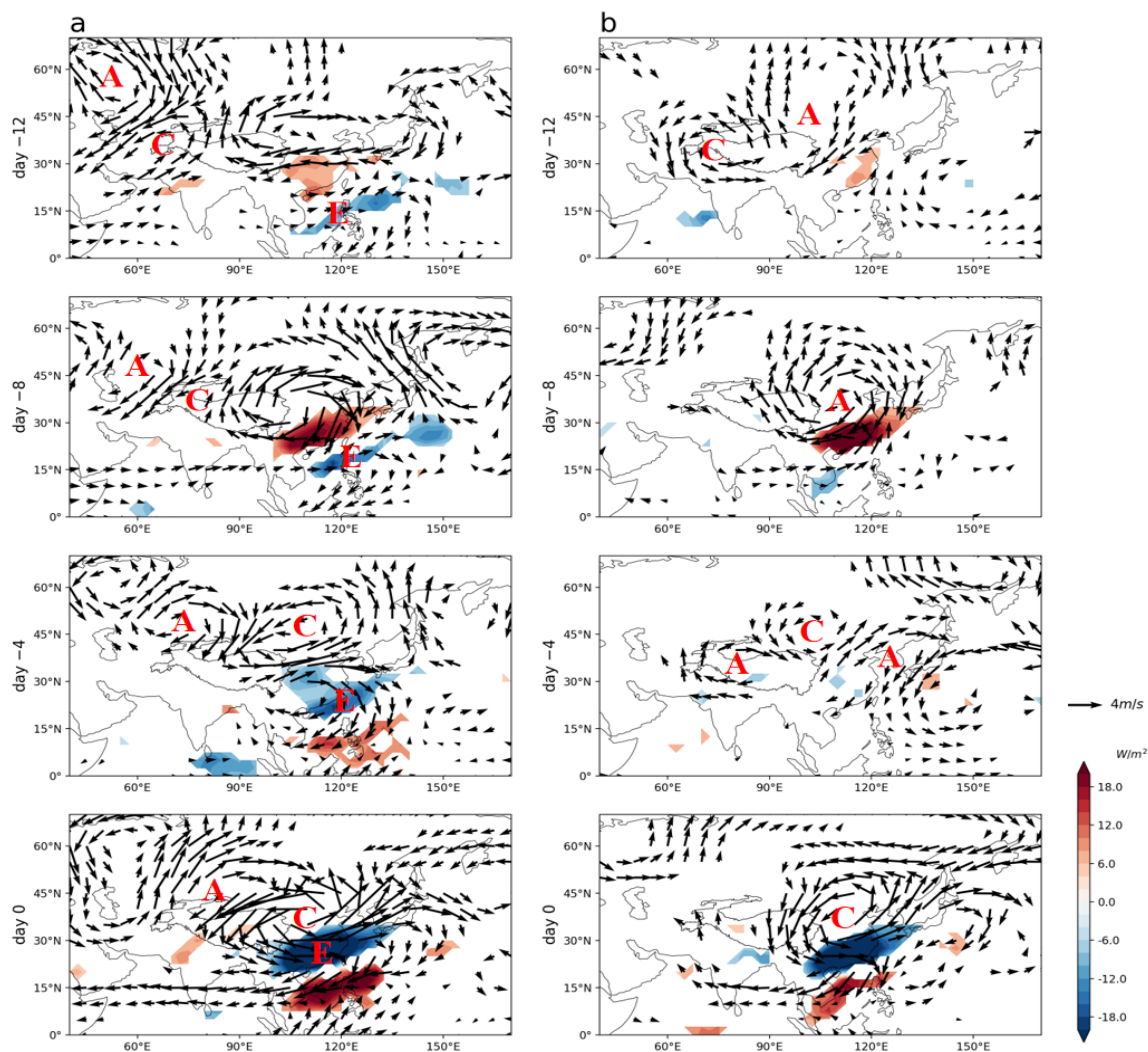
Fig. 5. Spatiotemporal structure of well- and poorly-predicted events of EASM ISV. Time lagged-composite maps, from Day -12 to Day 0 using four-day time increments, of 12–40-day filtered OLR anomalies (shading) and 200-hPa wind anomalies (vector) with respect to a 98 well-predicted and b 130 poorly-predicted ISV events based on ECMWF prediction for boreal summers of 1999–2018. Day 0 denotes the peak of each event, and the signs of dry events are reversed for composite. Only significant ( p < 0.05 ) OLR and wind anomalies based on the Student's t -test are shown. Letters A and C track the centers of the anomalous extratropical anticyclone and cyclone, respectively, whereas E tracks the center of enhanced tropical convection, as indicated by the negative OLR anomaly.
