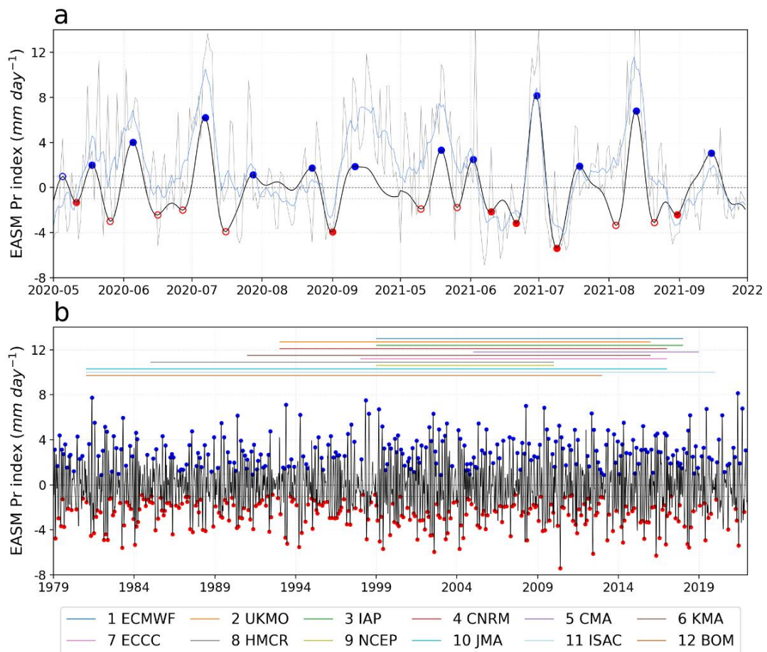
Fig. 2. Selection of ISV events from observations. Time series of EASM precipitation index anomaly (gray line), its 12–40-day component (black line), and seven-day running mean (blue line) for a 2020–2021 summers and b 1979–2021 summers in the observation of CPC. Blue and red dots denote centers (Day 0) of wet and dry ISV events, respectively. An ISV event is defined when the extrema of the 12–40-day filtered EASM precipitation index anomaly are > 0.5 standard deviation units for a wet event or < -0.5 standard deviation units for a dry event; events (circles) having a raw weekly precipitation index centered at Day 0 below the climatology for wet events, and above the climatology for dry events, are removed (see Methods). The hindcast periods of the 12 S2S models are also listed, represented by colored horizontal lines in b .
